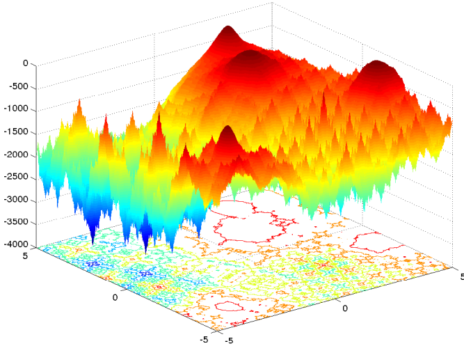
Fig. 11. Composition Function 3.
