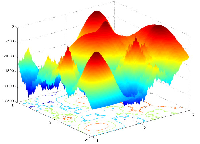
Fig. 9. Composition Function 1.
