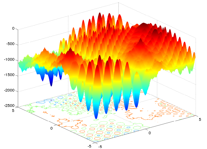
Fig. 10. Composition Function 2.
